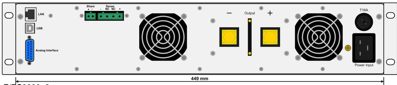
E/PS9000_2u_rear
