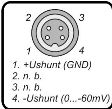
EPS/HC Shunt
