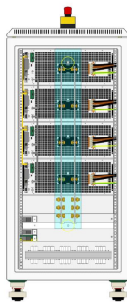
E/PSI 1200_Cabinet rear 120kW
