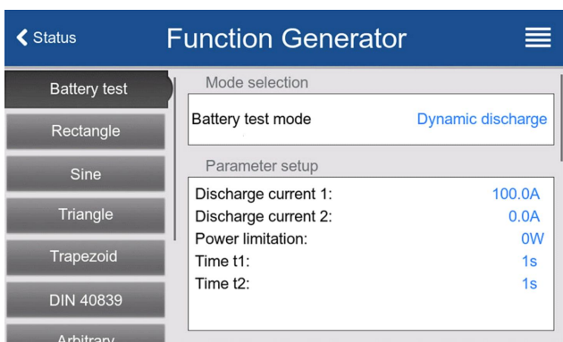
EPS/FG dynamic-discharge-function
