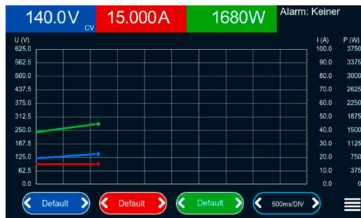
EPS 1000 Graph (HMI)
