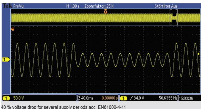
40 % voltage drop for several supply periods acc. EN61000-4-11
