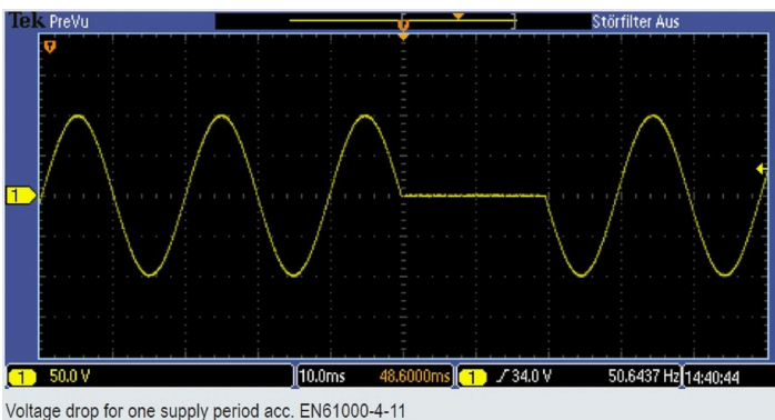
EPS/ACS Voltage drop EN61000-4-11
