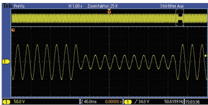
40 % voltage drop for several supply periods acc. EN61000-4-11 EPS/ACS 40% Voltage drop EN61000-4-11
