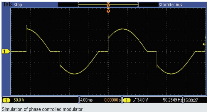
Simulation of phase controlled modulator EPSACS Simulation Ph. control modulator
