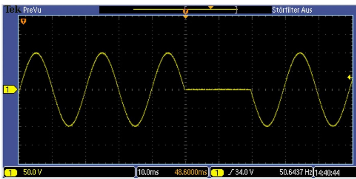
Voltage drop for one supply period acc. EN61000-4-11 EPS/ACS Voltage drop EN61000-4-11
